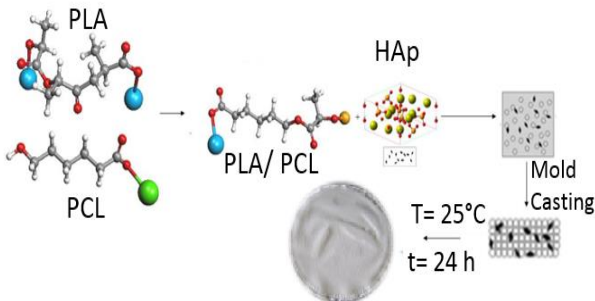
Figure 1: Schematic representation of synthesis route of composite.
