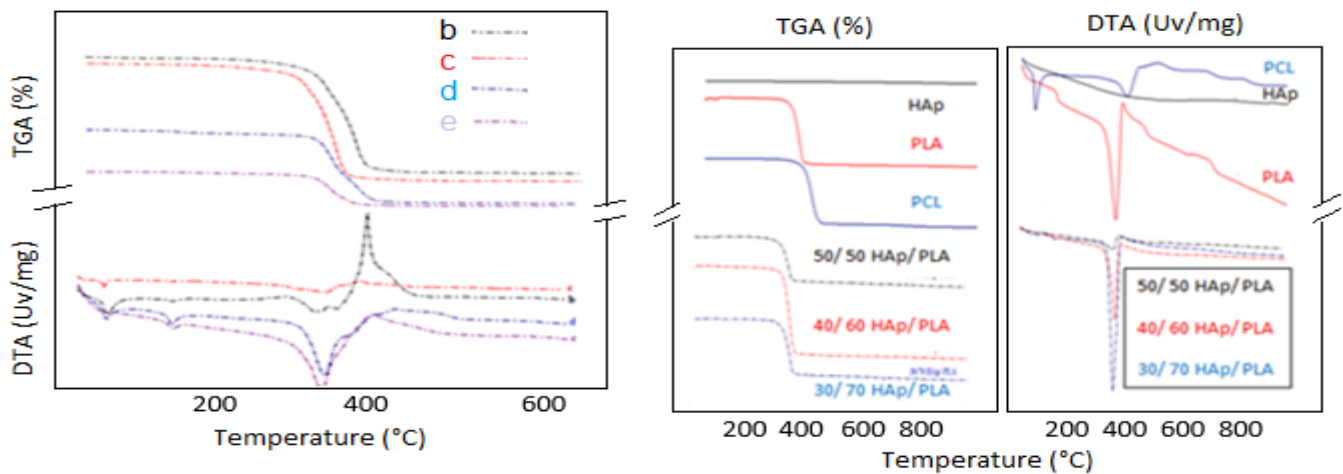
Figure 6: TGA (1) and DTA (2) curves of the composites HAp i / PLA and HAp i / PLA / PCL, with molar ratios of b = 50/30/20, c =50/10/40 d = 50/20/30 and e =50/40/10 (Heating rate: 10 °C / min).
