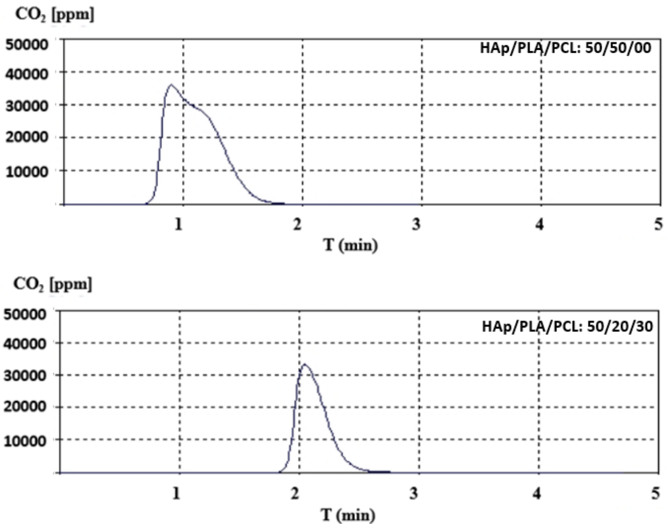
Figure 9: Plot of TOC vs. time for HAp t / PLA/PCL composite scaffold with a molar ratio of a = 50/50/00 and b =50/20/30.
