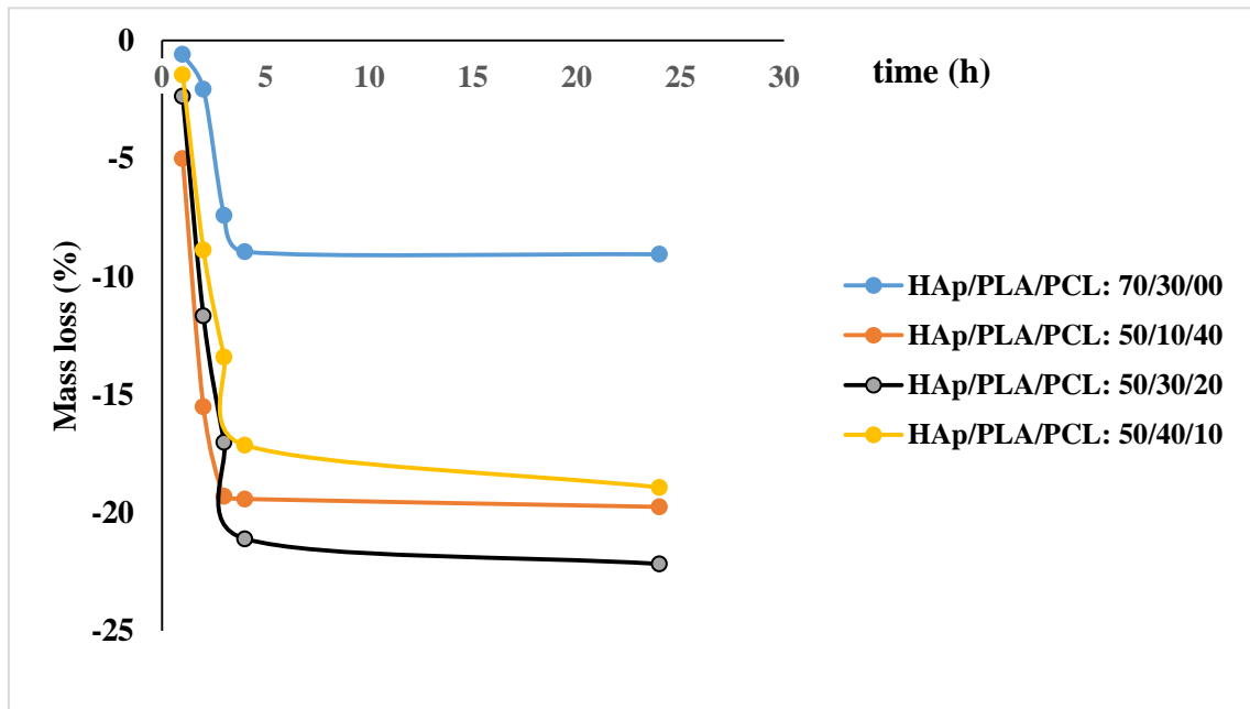
Figure 7: Biodegradability at 37 ° C of membranes HAp i /PLA/PCL in PBS
