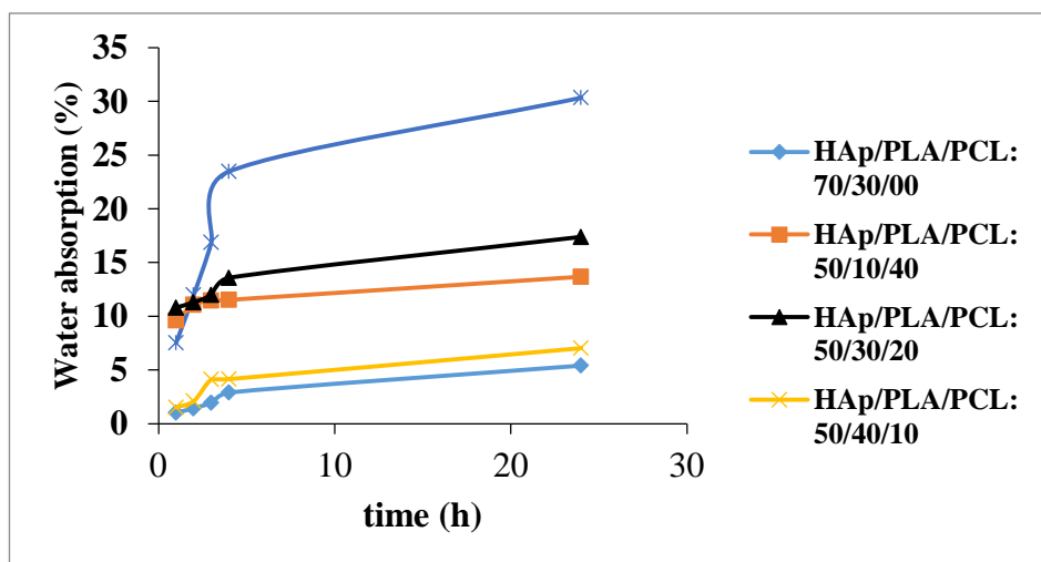
Figure 8: Swelling ratio of composite HAp i /PLA/PCL.
