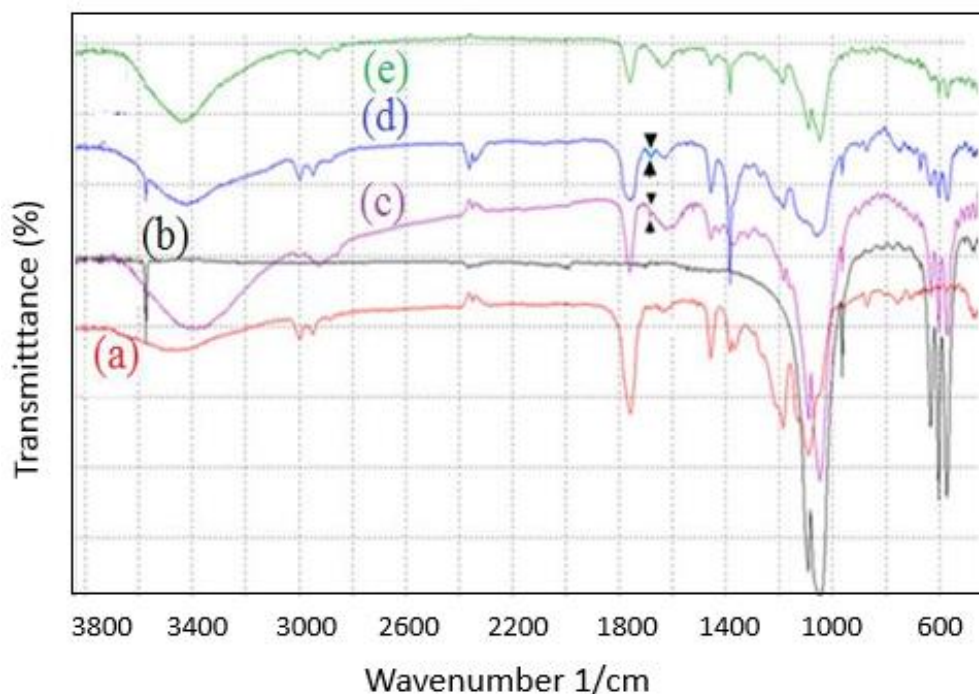
Figure 2: FTIR spectra of the HAp/PLA composite, with molar ratios: a=PLA, b= HAp, c = 70/30, d =60/40 and e=50/50.
