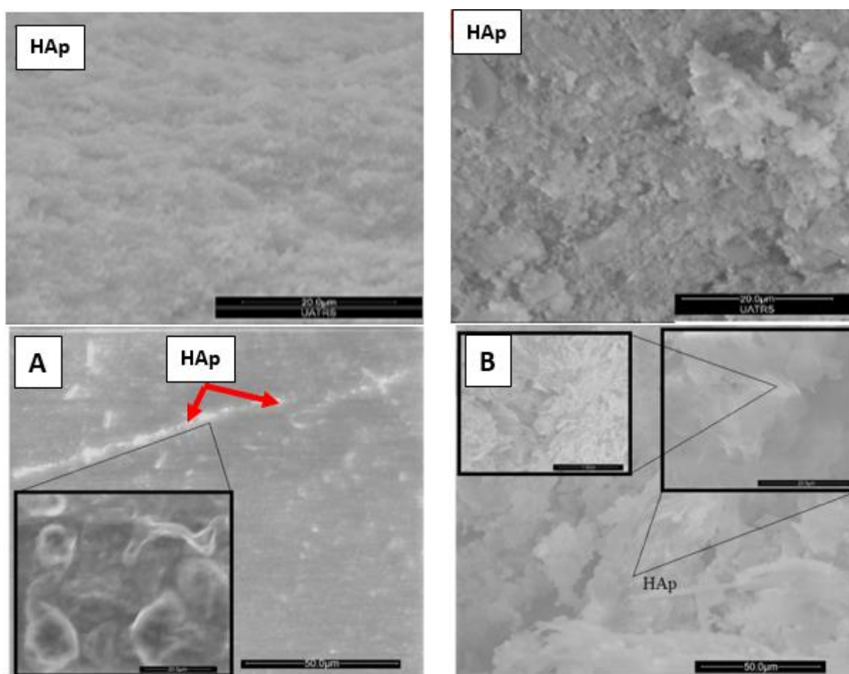
Figure 4: SEM micrographs of two membranes surfaces of HAp t /PLA/PCL with a molar ratio of a = 50/50/00 and b =50/20/30.
