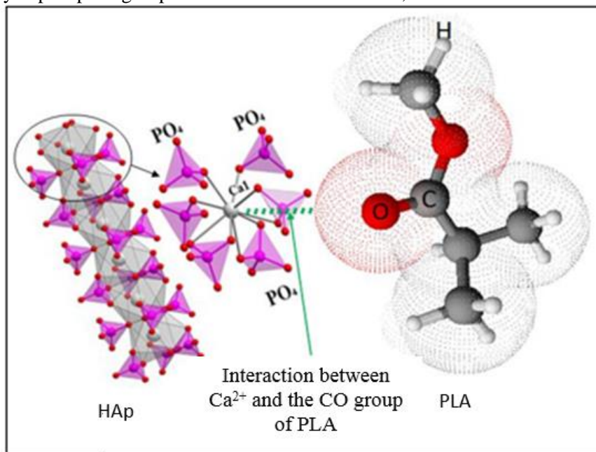
Figure 3: A schematic model of the complexation between the carboxyl groups of PLA and \text{Ca}^{2+} of HAp t .
