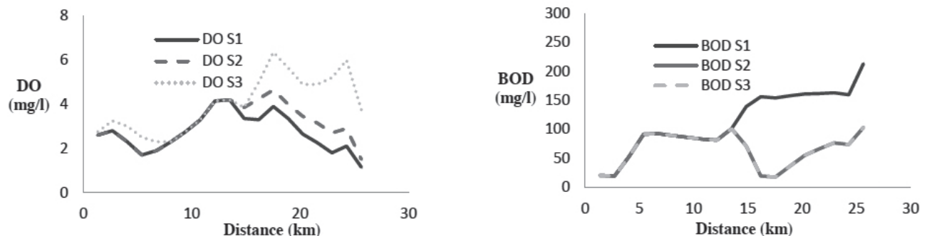
Figure 6. Modeling results of water quality parameters (DO and BOD) in Zimar stream for the current situation
