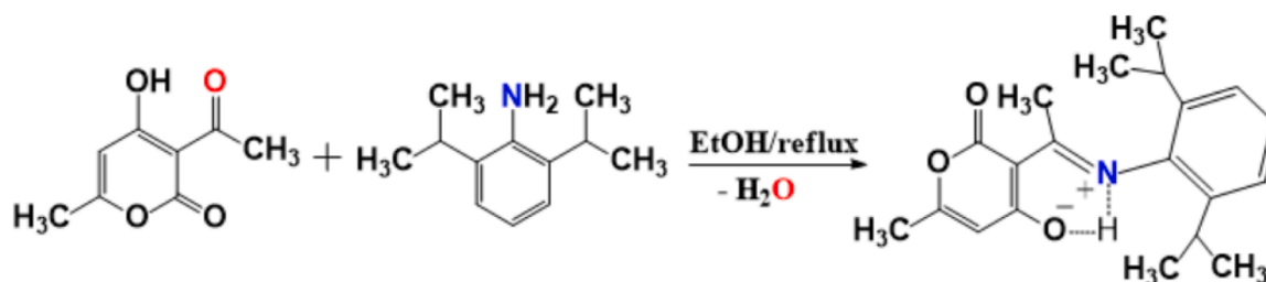
Scheme 1. Preparation of the desired Zwitterion Schiff base.
