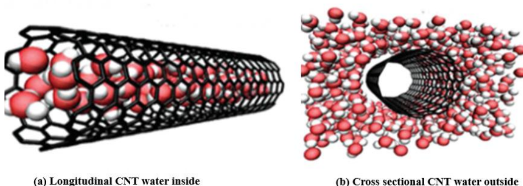
Figure 4. Schematic showing how water molecules interact with CNT armchair surfaces. (a) Longitudinal CNT water inside and (b) cross-sectional water outside CNT armchair views. Reproduced with permission from ACS [60].
