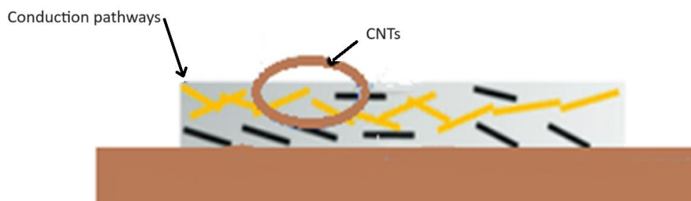
Figure 3. Schematic describing CNT conductive network formation in water.
