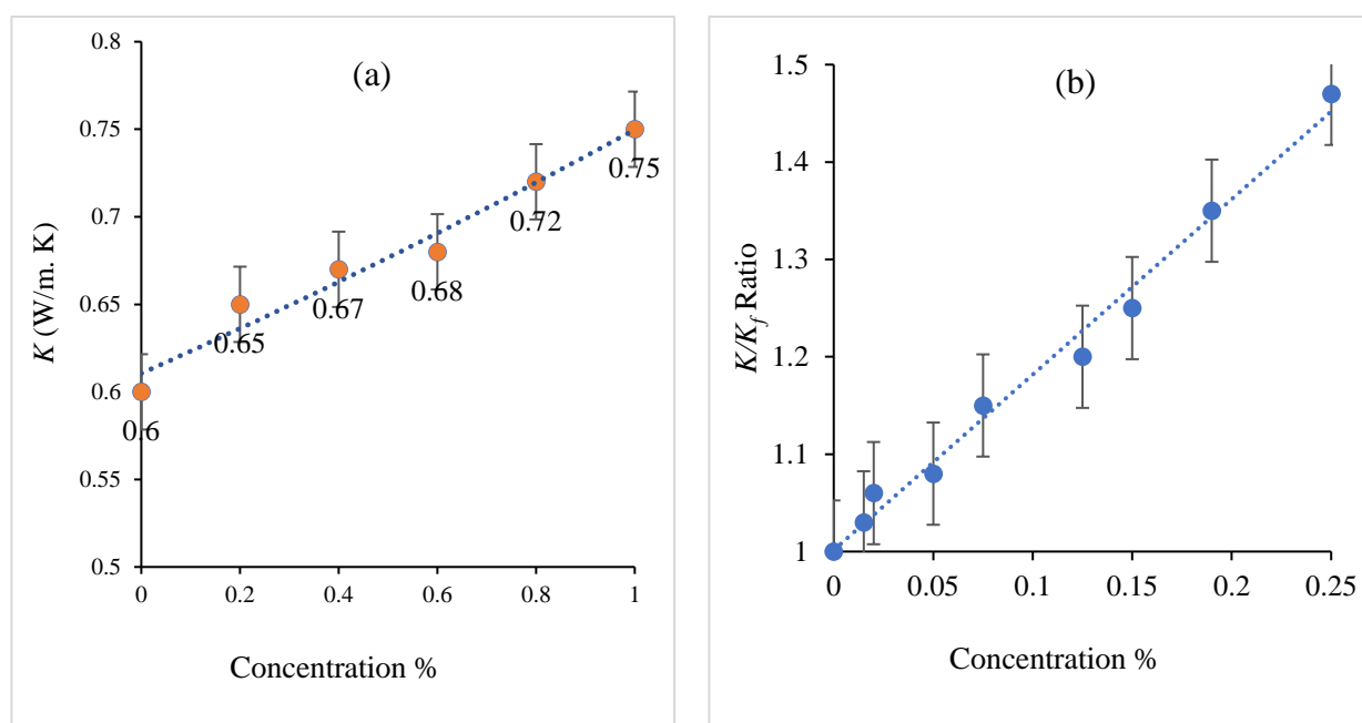
Figure 6. Effect of CNT concentration on aqueous nanofluid thermal conductivity. (a) Thermal conductivity values vs. MWCNT concentration, reproduced with permission from ACS [89]. (b) Simulated thermal conductivity improvement compared to water value, reproduced with permission from Hindawi open access [90].
