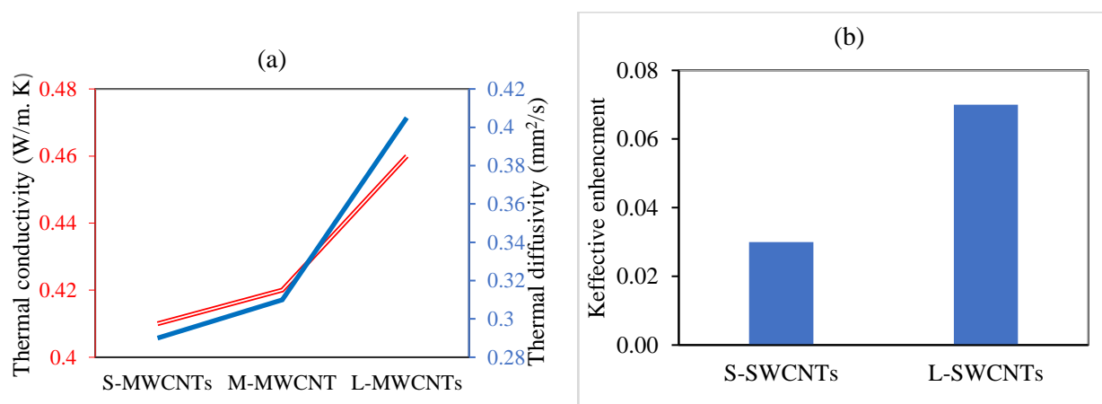
Figure 7. Effect of aspect ratio on CNT aqueous nanofluid thermal conductivity. (a) MWCNT length effect (having 10% concentration), reproduced with permission from MDPI open access [33]. (b) Thermal conductivity enhancement by using SWCNTs (short vs. long tubes), reproduced from Yildiz Technical University open access [19]. The starting letter S-, M- and L- describe short, medium and long CNTs, either MWCNTs in (a) or SWCNTs in (b).
