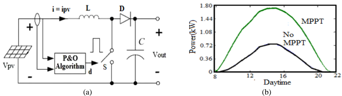
Figure 4. DC/DC boost-converter controlled by (a) MPPT control scheme, and (b) its validation
