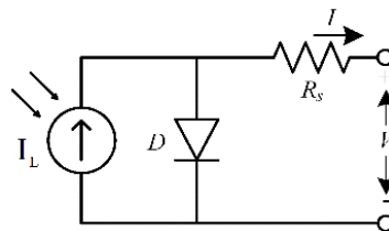
Figure 2. One-diode PV cell equivalent circuit model
