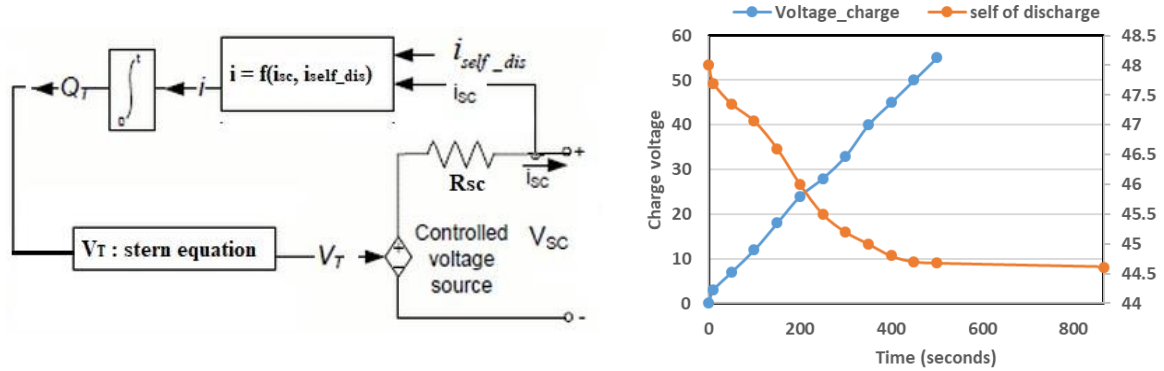
Figure 9. Modeling and validation of super-capacitor SC: (a) Equivalent electrical circuit of SC, and (b) its performance during charging and self-discharging
