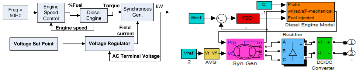
Figure 7. Modeling of DG: (a) Schematic of DG model, and (b) MATLAB/Simulink simulation model
