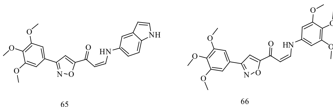
Figure 30. Arylamino-isoxazolyl-2-propenone derivatives
