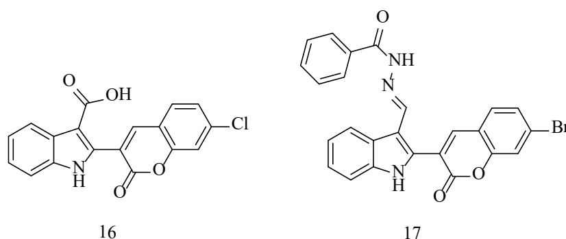
Figure 8. Indole-coumarin hybrid compounds
