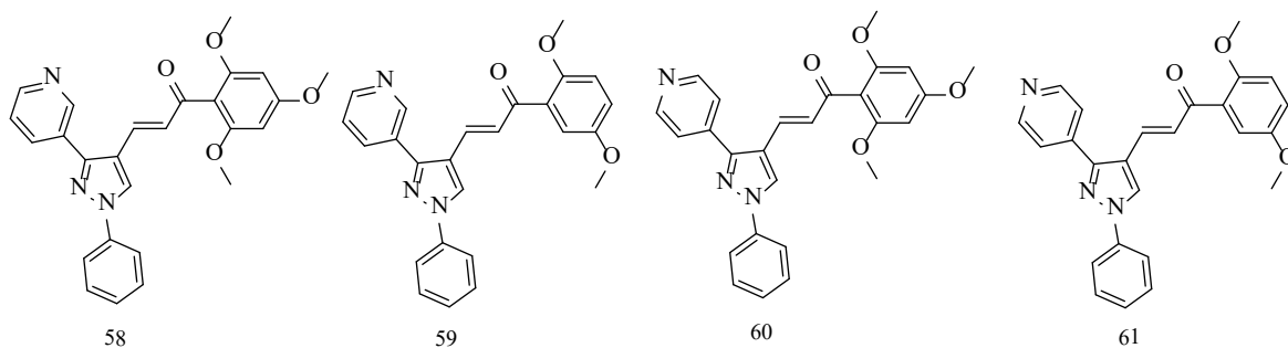
Figure 27. Pyrazolic-chalcone derivatives
