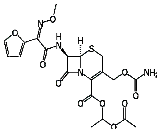
Figure (1): Chemical structure of cefuroxime axetil.
