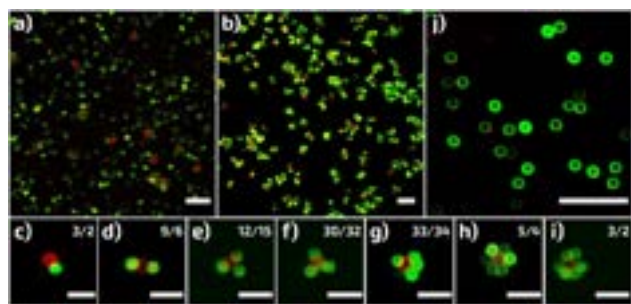
Fig. 2 Confocal fluorescence microscopy images of clusters obtained by incubating 1.6\ \mu\text{m} \text{TPM}_A \sim \text{Ink}_{565} and 1.5\ \mu\text{m} \text{PS}_B particles in a 1 : 40 ratio (a) before and (b) after purification. (c)–(i) Zoom images of the different clusters containing 1 to 7 PS particles. Their relative amounts (in %) in the sample before/after purification are given at the top right corner of each image. (j) Confocal fluorescence microscopy image of the patchy PS particles resulting from the strand-displacement disassembly of \text{TPM}_A \sim \text{Ink}_{565} \sim \text{PS}_B clusters. Scale bar of 10\ \mu\text{m} for (a), (b) and (j), and 5\ \mu\text{m} for (c) to (i).
