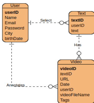
Fig. 2 The Entity Relationship Diagram.
